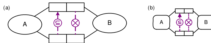
Figure 3 An example with set-comparison constraints in the old notation (a) and new notation (b).
