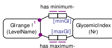
Figure 19 Textual constraints appear as footnotes in ORM 2.
